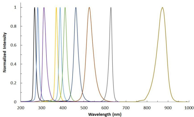
LEDs Included with LED-COMPLETE-KIT 265, 280, 310, 365, 385, 405, 470, 533, 635 and 880 nm Plus 3689K Broadband LED
