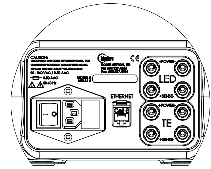
REAR VIEW SHOWING CONNECTIONS DETAIL A
